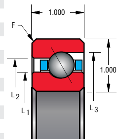
Circular pocket separator 1/2" balls
