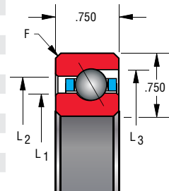
Circular pocket separator 3/8" balls
