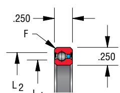
Snap-over separator 1/8" balls
