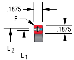
Snap-over separator 3/32" balls
