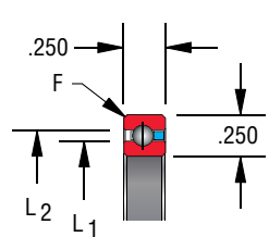
Snap-over separator 1/8" balls
