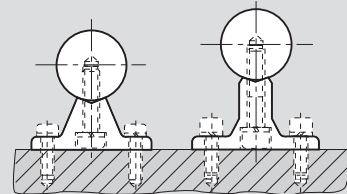
Conventional flanged designs
